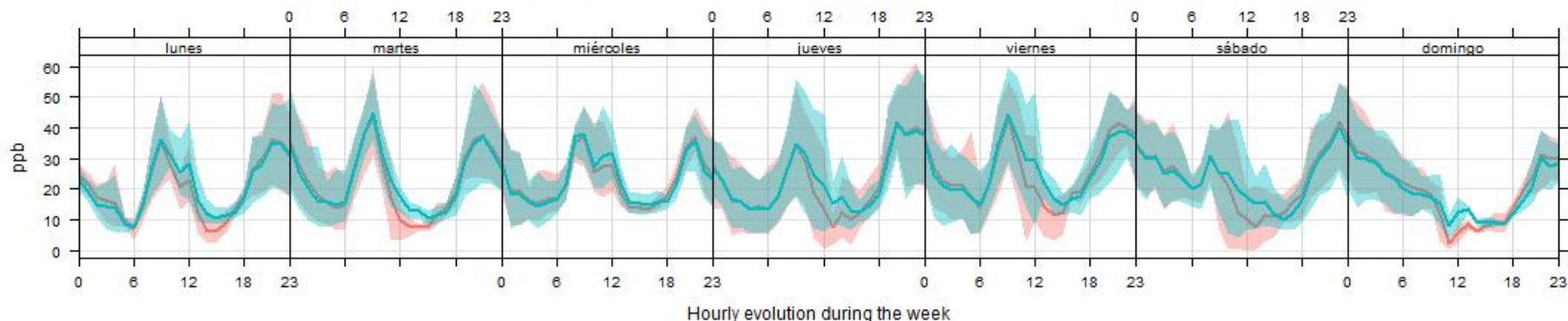
Time variation of Kunak Air V2 and Ref. Palau Reial : NO 2 GCc
