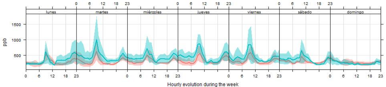
Time variation of Kunak Air V2 and Ref. Palau Reial : CO GCc
